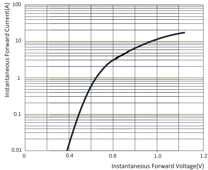
FIG3: Forward Voltage
